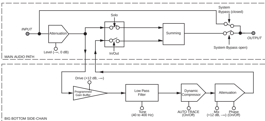
Block Diagram of Aphex Big Bottom Pro
