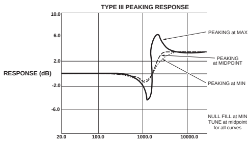
Peaking control
